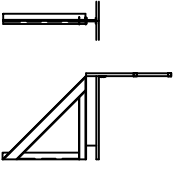
NORTH SIDE BRACE 6 REQUIRED
