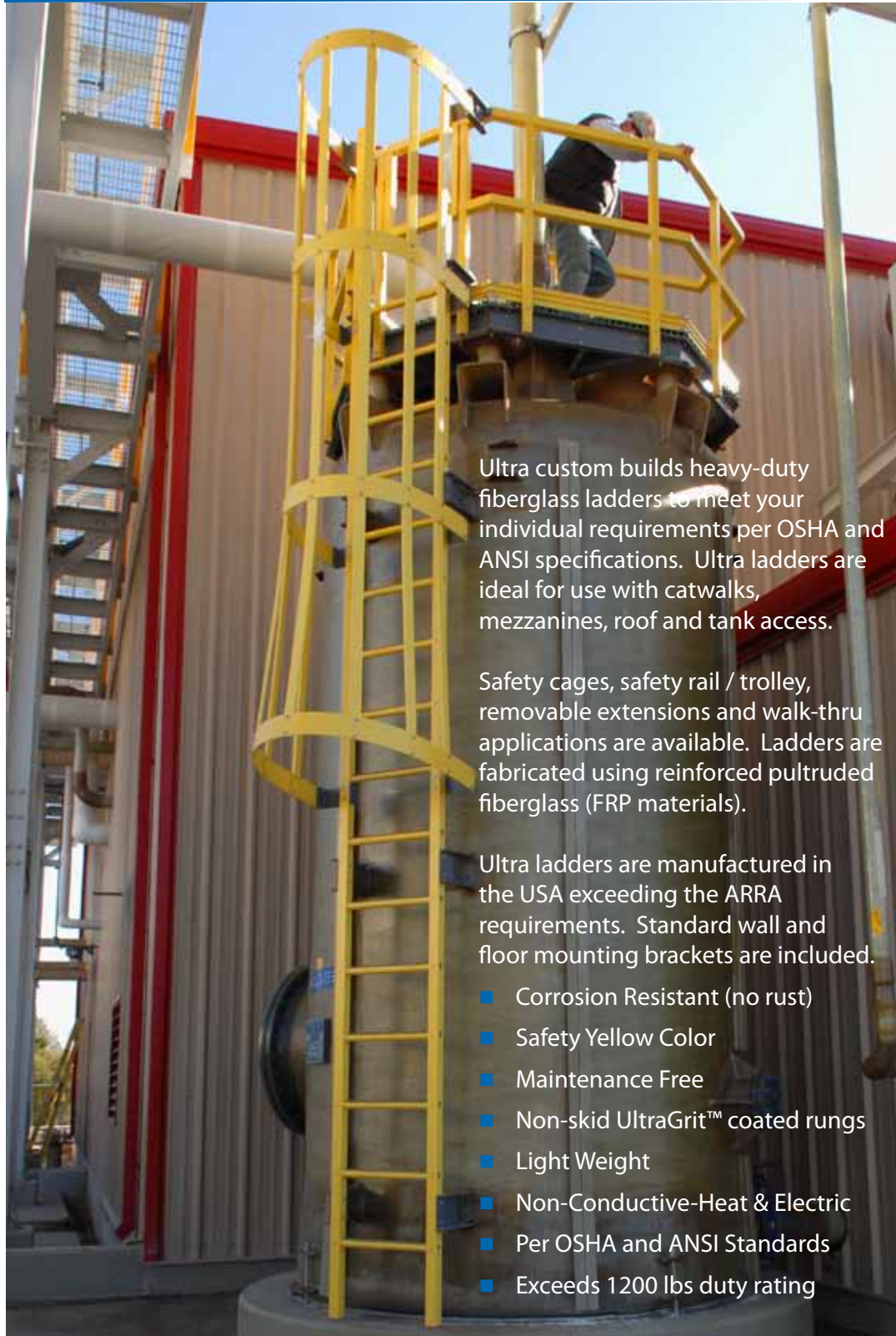
Non-skid UltraGrit™ coated rungs
